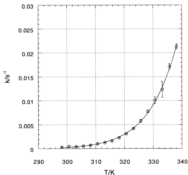
Figure 12. Exponential least-squares fit of first-order rate constants ( k ) versus temperature ( T ) to the Eyring equation k = (k_B T/h) \exp(-\Delta S^\ddagger/R) \exp(-\Delta H^\ddagger/RT) for the reaction (\mu\text{-}^{15}\text{N}_2)\{\text{Mo}[\text{N}(\text{R})\text{Ar}]_3\}_2 \rightarrow 2 \text{ }^{15}\text{NMo}(\text{N}[\text{R}]\text{Ar})_3 . Activation parameters obtained from the fit are \Delta H^\ddagger = 22.6 \pm 0.3 \text{ kcal}\cdot\text{mol}^{-1} and \Delta S^\ddagger = 0.4 \pm 1.1 \text{ cal}\cdot\text{mol}^{-1}\cdot\text{K}^{-1} .
