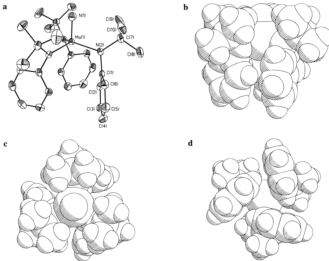
Figure 14. (a) Structural diagram and atom-labeling scheme for \text{NMo}[\text{N}(t\text{-Bu})\text{Ph}]_3 . Thermal ellipsoids are at the 35% probability level. Selected bond lengths (Å) and angles (deg) for \text{NMo}[\text{N}(t\text{-Bu})\text{Ph}]_3 are as follows: \text{Mo}(1)\text{--N}(1) , 1.658(5); \text{Mo}(1)\text{--N}(2) , 1.979(2); \text{C}(1)\text{--N}(2) , 1.444(4); \text{N}(2)\text{--C}(7) , 1.513(3); \text{N}(1)\text{--Mo}(1)\text{--N}(2) , 102.94(7); \text{N}(2)\text{--Mo}(1)\text{--N}(2') , 115.13(5); \text{C}(1)\text{--N}(2)\text{--C}(7) , 117.3(2); \text{C}(1)\text{--N}(2)\text{--Mo}(1) , 113.5(2); \text{C}(7)\text{--N}(2)\text{--Mo}(1) , 128.2(2). Space-filling representations of \text{NMo}[\text{N}(t\text{-Bu})\text{Ph}]_3 viewed (b) perpendicular to the nitrido bond axis, (c) along the nitrido bond axis facing the hemisphere protected by tert -butyl groups, and (d) along the nitrido bond axis facing the hemisphere protected by phenyl groups.
