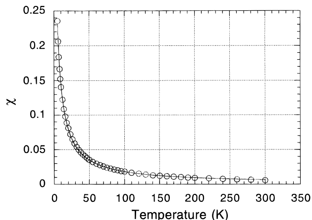
Figure 1. SQUID magnetic susceptibility data for solid \text{Mo}[\text{N}(\text{R})\text{Ar}]_3 from 5 to 300 K fit to the Curie–Weiss law ( \mu = 3.82\ \mu_{\text{B}} ; see Experimental Section for details).
